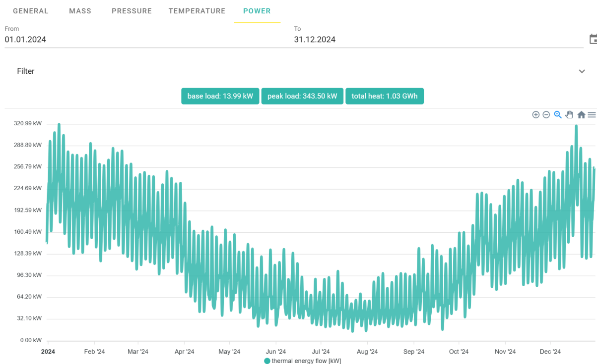
Figure 52: Thermal energy flow at one consumer.
