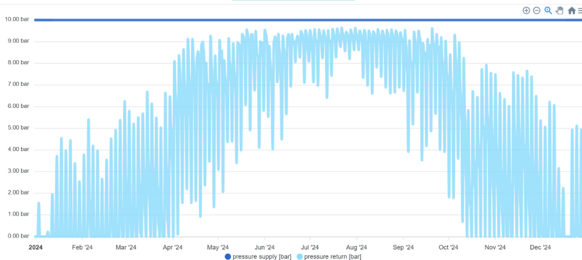
Figure 46: Pressure supply and return load curves at the producer.
