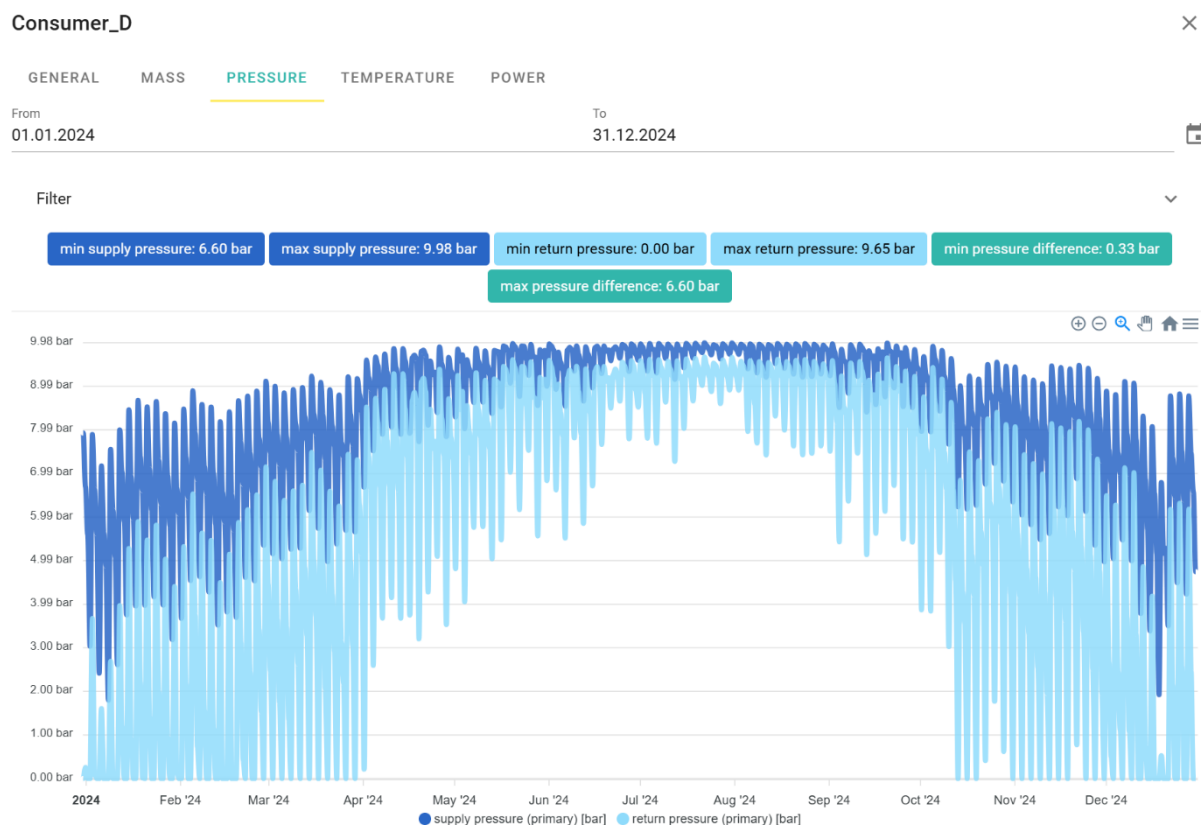
Figure 50: Pressure supply and pressure return load curves at one consumer.
