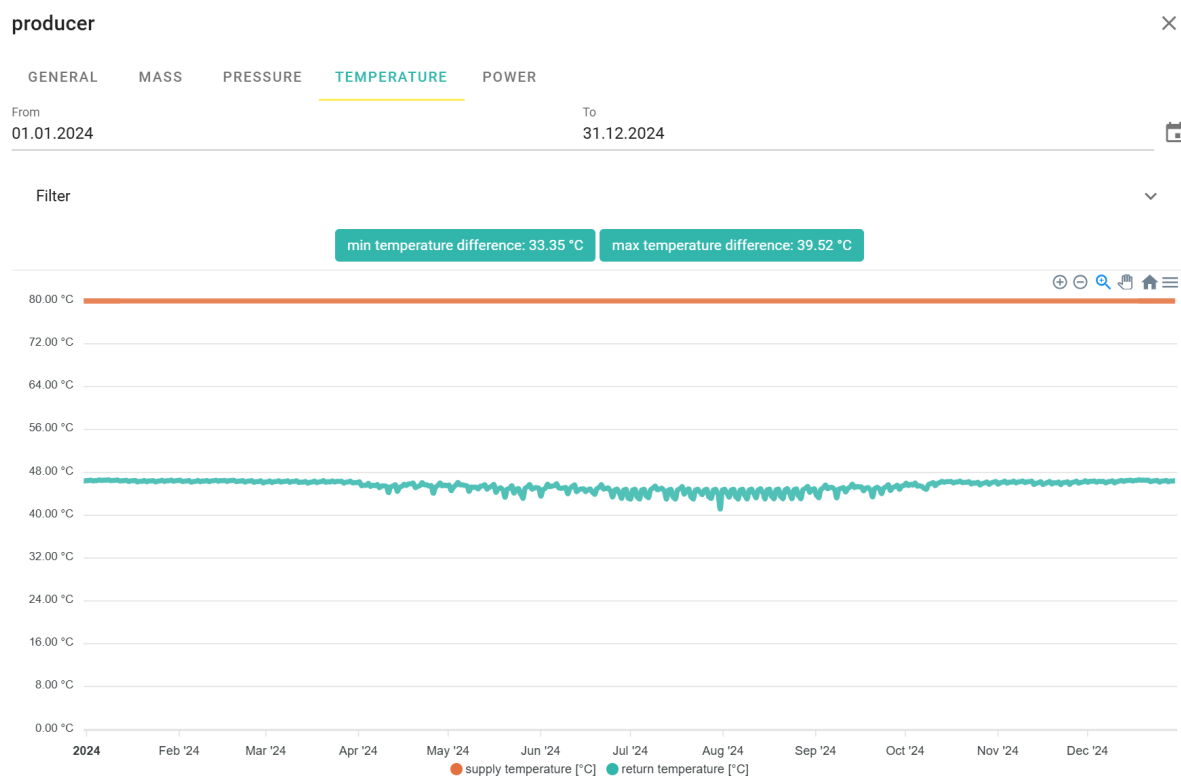
Figure 28: Temperature load curve on the producer.
