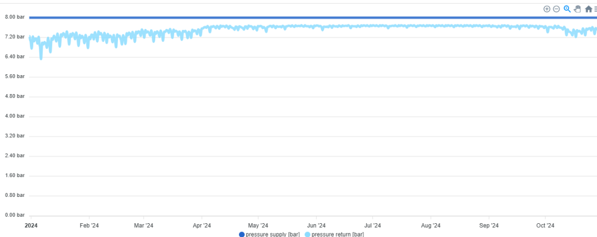
Figure 17: Producer pressure supply and pressure return curves.
