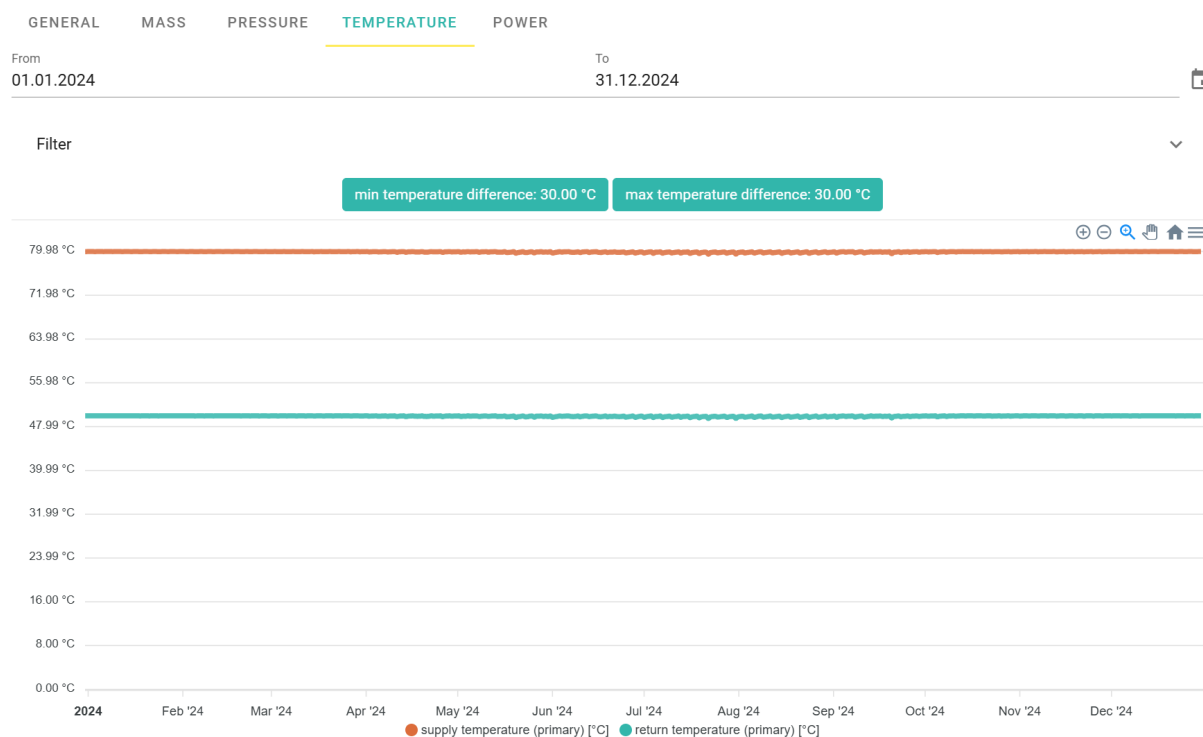
Figure 51: Temperature supply and return load curves at one consumer.
