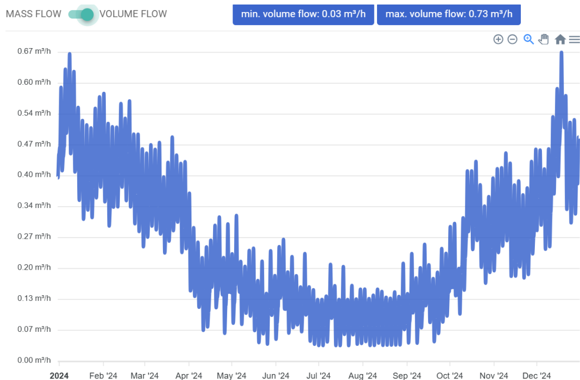
Figure 6: Consumer mass flow rates yearly simulation results.
