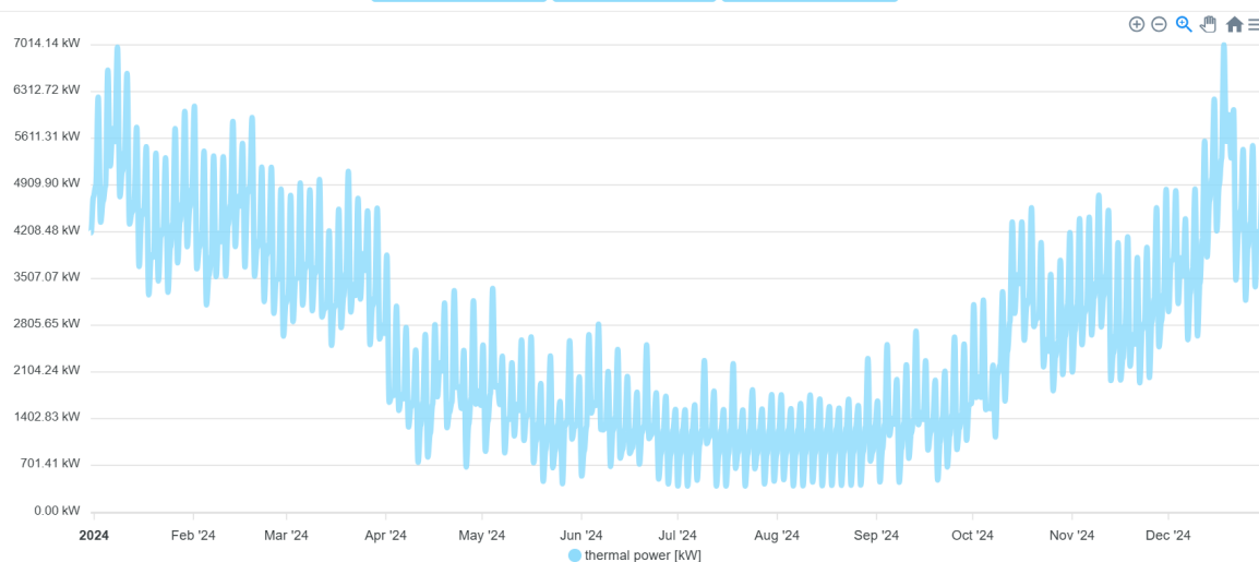
Figure 29: Power generation load curve at the producer.
