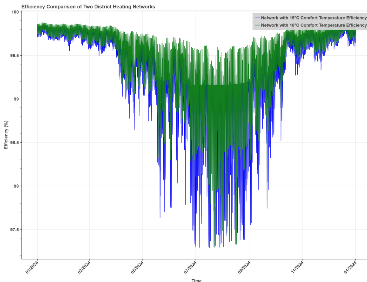
Figure 54: Efficiency plot of two district heating networks.
