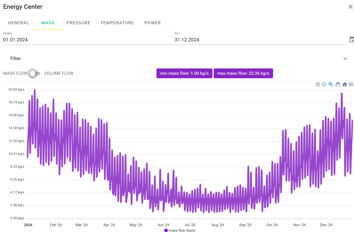
Figure 35: Mass flow load curve at the producer.
