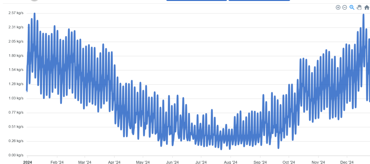
Figure 49: Mass flow load curve at one consumer.
