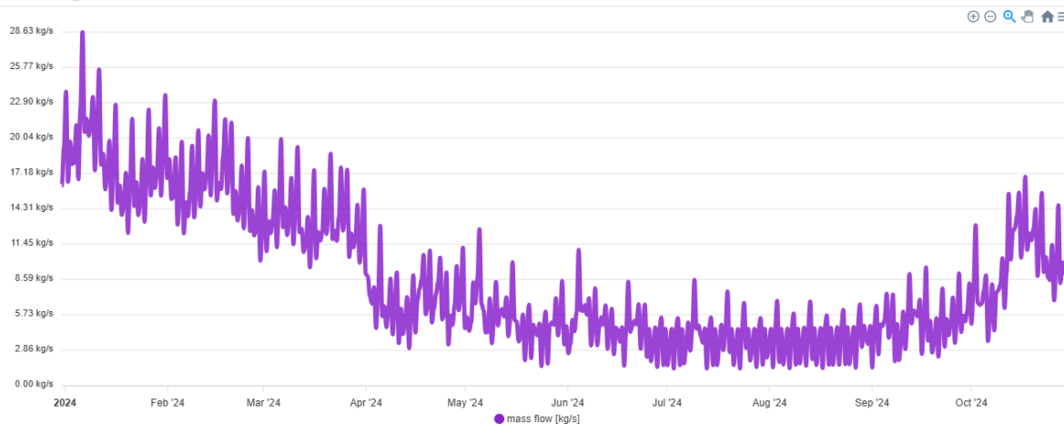
Figure 16: Producer mass flow load curve.
