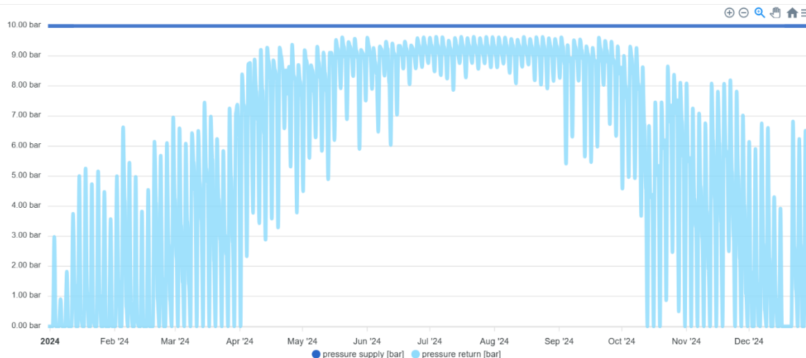
Figure 36: Pressure return and supply load curves at the producer.
