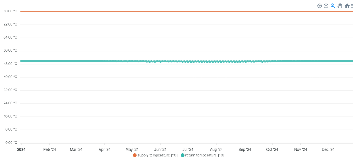
Figure 37: Temperature supply and return load curves at the producer.
