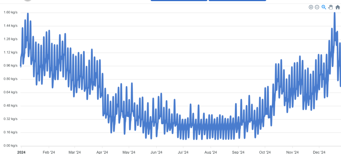
Figure 30: Mass flow load curves at one consumer.
