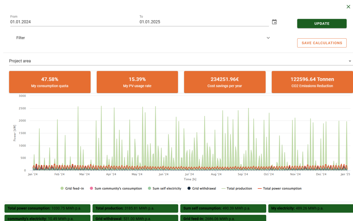
Figure 56: Yearly building power calculation in Bari.
