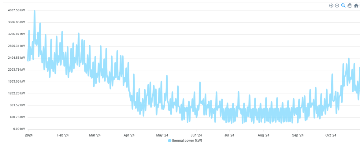
Figure 19: Power generation load curve at the producer.
