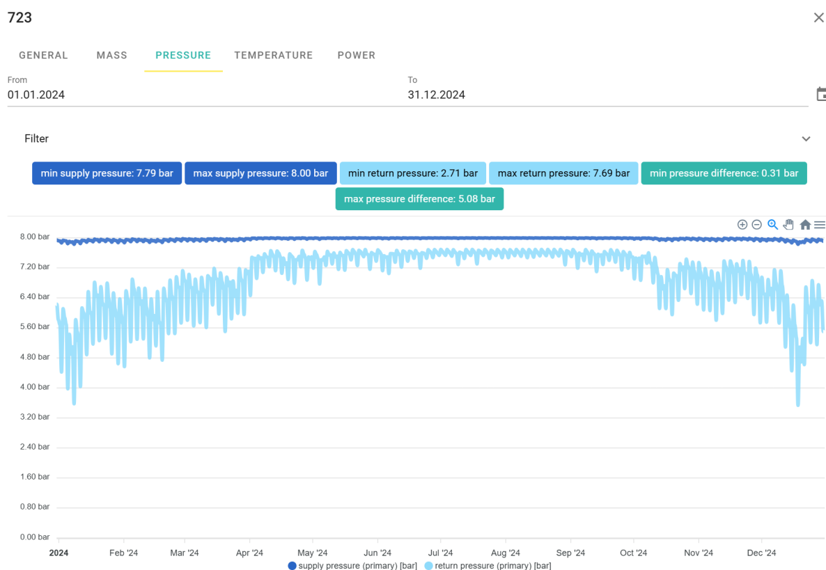
Figure 31: Pressure return and supply at one consumer.
